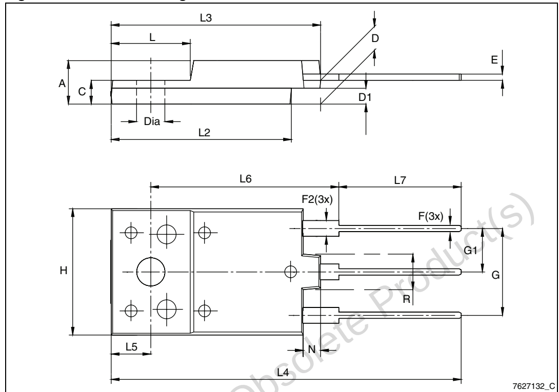
Figure 19. TO-3PF drawing
