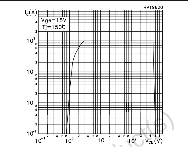
Figure 15. Turn-off SOA
